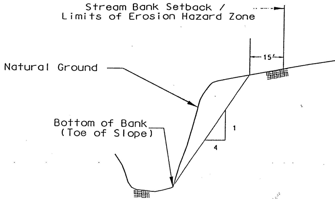
Figure 3.6.3-1 Minimum Erosion Control Setback
